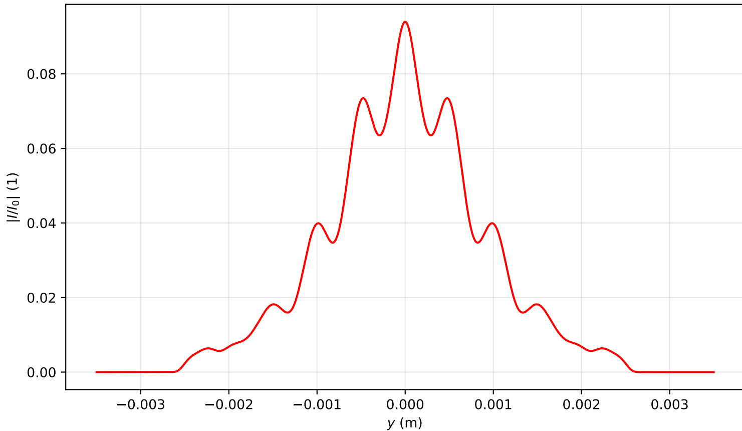
Intensity profile I(x=0, y, z=3.344)/I_0 , P_{in}=2.0P_{cr} , artificial time
